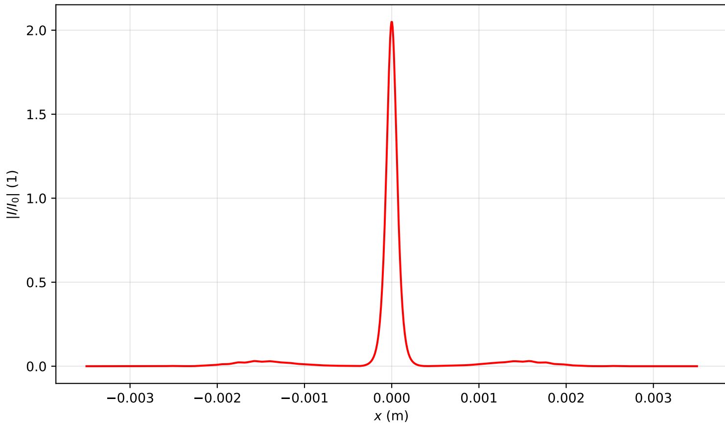
Intensity profile I(x, y = 0, z = 1.274)/I_0 , \text{Pin}=8.0\text{Pcr} , artificial time
